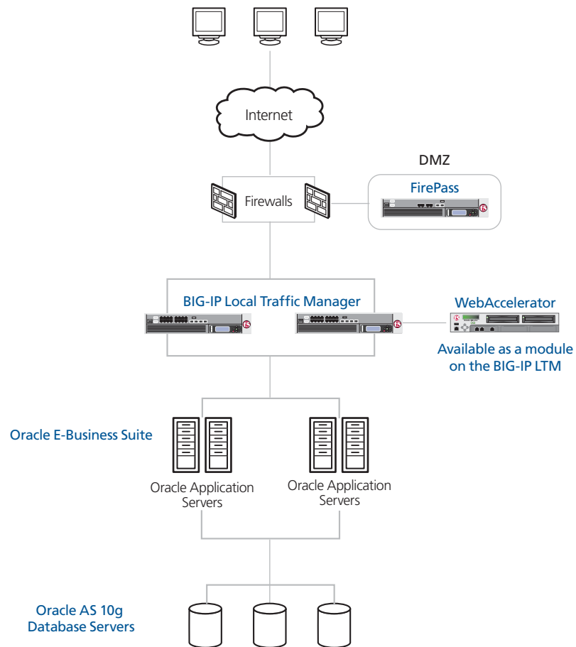
Figure 1.1 BIG-IP Oracle E-Business Suite logical configuration example
